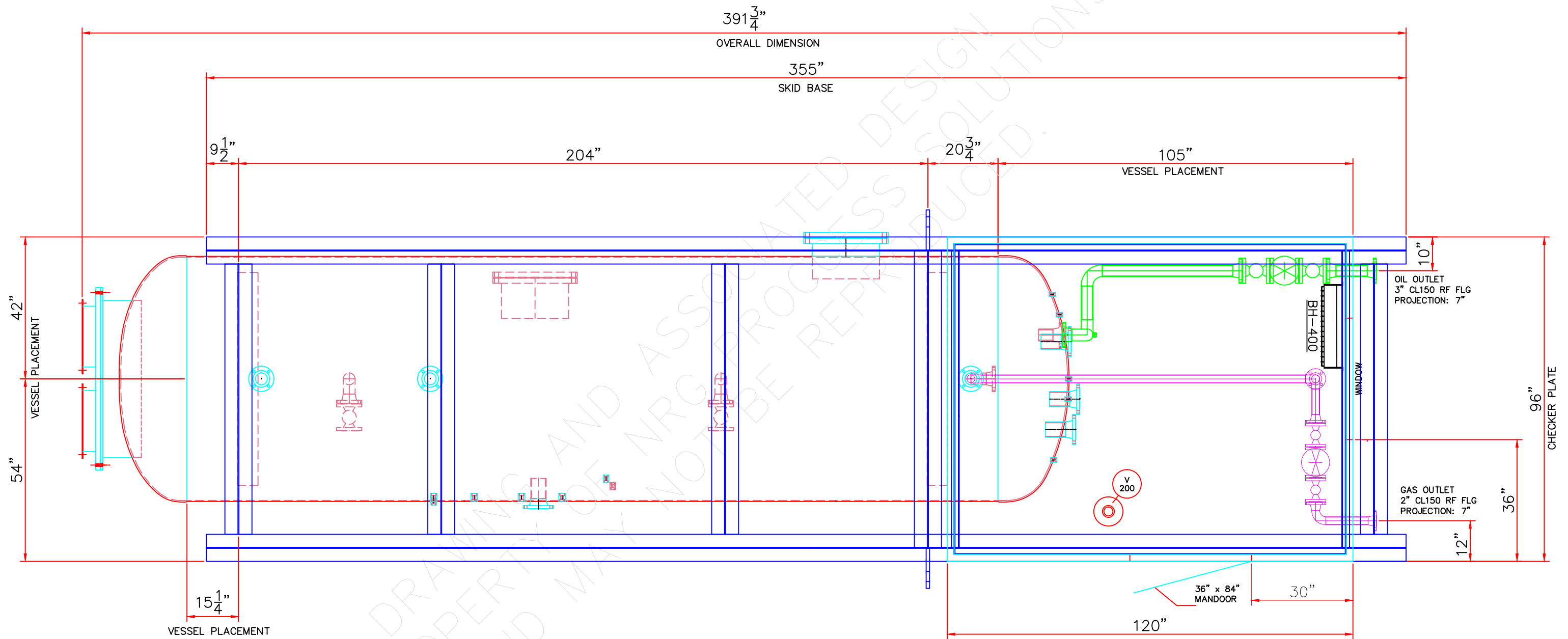
PLAN VIEW 1
