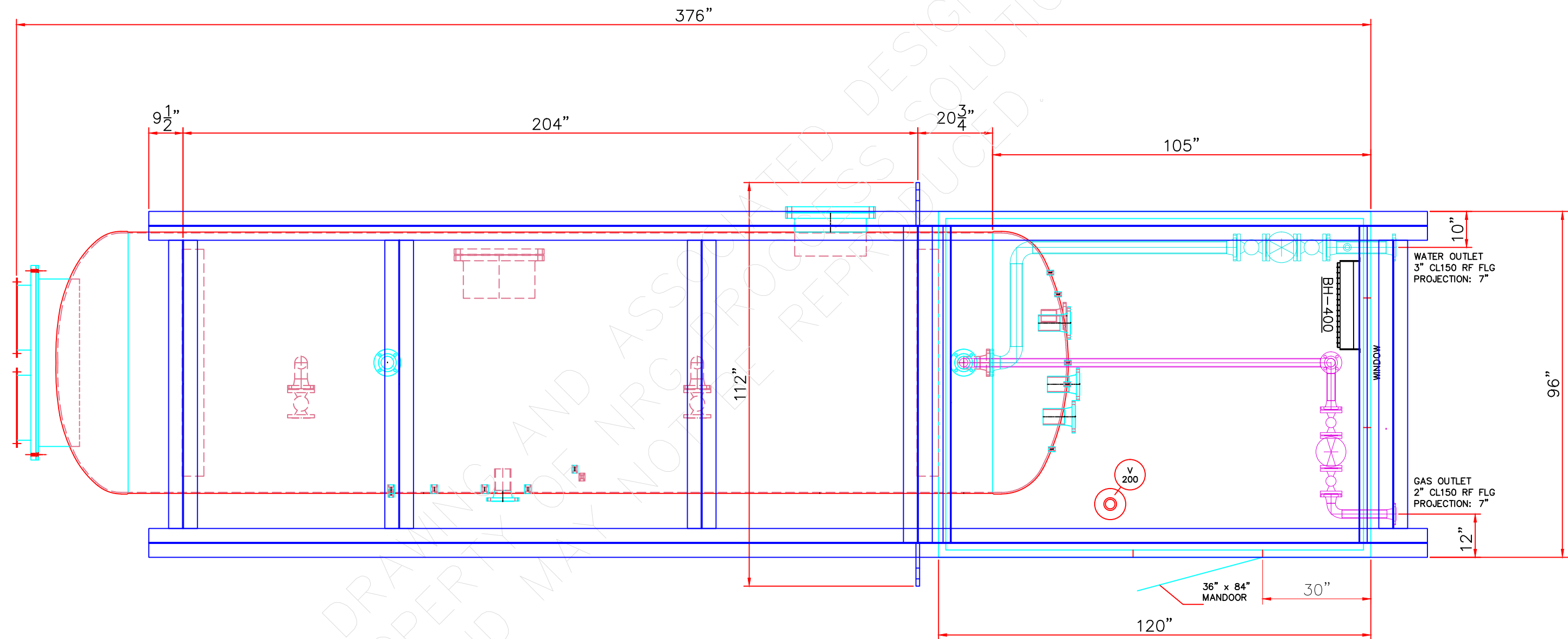
PLAN VIEW 2
